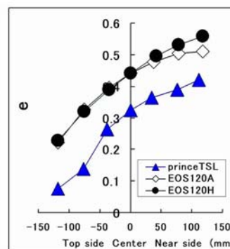
Fig. 10 Predicted rebound power coefficient.
