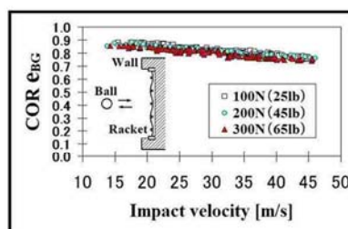
(a) Measured COR
