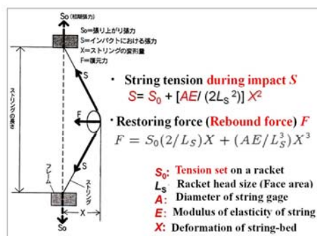
Fig. 3 Deformation, tension, restoring force during impact.
