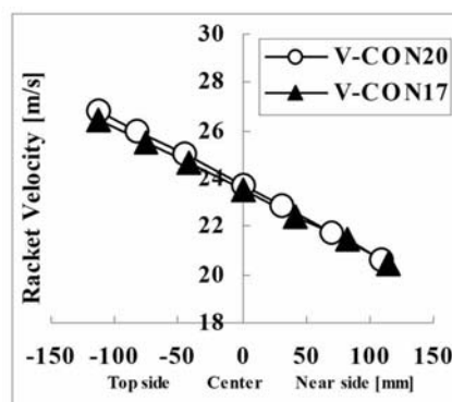
Fig. 24 Predicted Pre-impact racket head velocity V_{Ro} ( N_s = 56.9 \text{ Nm} , V_{BO} = 10 \text{ m/s} )
