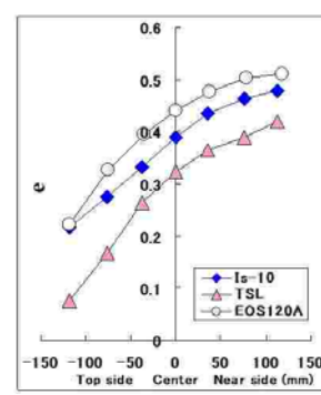
Fig. 30 Predicted rebound power coefficient e ( N_s = 56.9 \text{ Nm} , V_{B0} = 10 \text{ m/s} )
