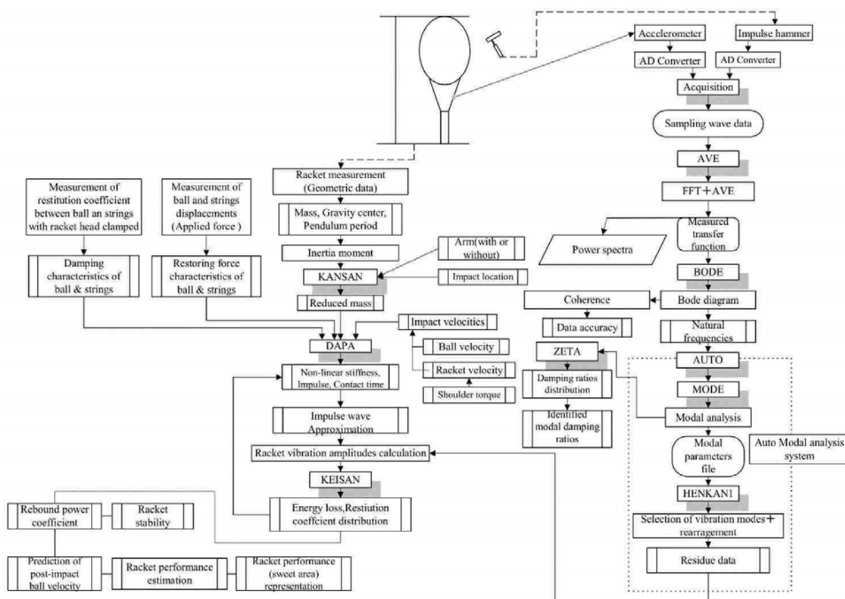
Fig. 7 Computer aided prediction and estimation system for tennis racket performance in terms of power.
