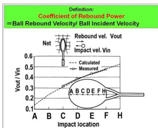
Fig. 8 Definition of coefficient of rebound power : Ball Rebound Velocity / Ball Incident Velocity
