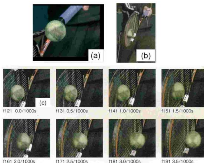
Fig. 9 The impact behavior between the racket and ball in tennis topspin shots (ball speed and spin generation)
