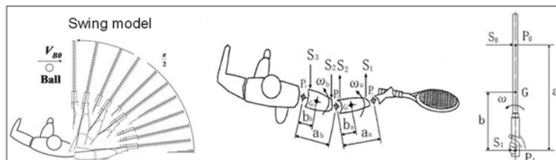
Fig. 6 Player's forehand stroke swing model for the prediction of racket power
