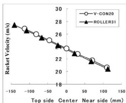
Fig. 16 Pre-impact head velocity.
