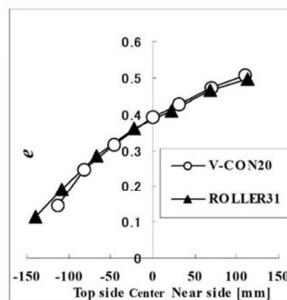
Fig. 17 Rebound power coefficient e ( N_s = 56.9 \text{ Nm} , V_{B0} = 10 \text{ m/s} )
