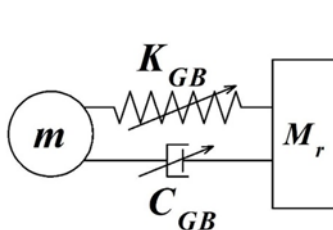
Fig. 5 Non-linear Impact model of a ball-string bed system.
