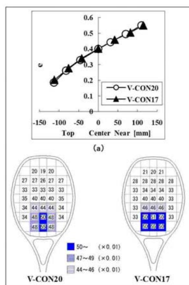
Fig. 25 Rebound power coefficient e ( N_s = 56.9 \text{ Nm} , V_{BO} = 10 \text{ m/s} )
