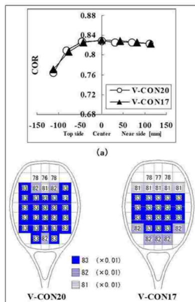
Fig. 23 Predicted Restitution coefficient e_r ( N_s = 56.9 \text{ Nm} , V_{BO} = 10 \text{ m/s} )
