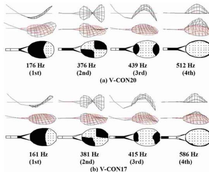
Fig. 21 Experimentally identified vibration modes.
