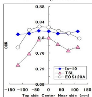
Fig. 29 Predicted Restitution coefficient e_r ( N_s = 56.9 \text{ Nm} , V_{B0} = 10 \text{ m/s} )
