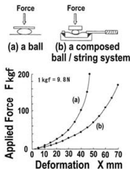
Fig. 1 Applied force- deformation test
