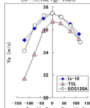
Fig. 31 Predicted post-impact ball velocity V_B ( N_s = 56.9 \text{ Nm} , V_{B0} = 10 \text{ m/s} )
