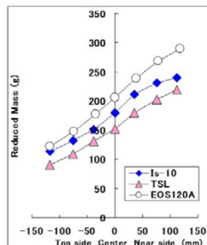
Fig. 28 Reduced mass M_r of racket at the hitting locations.
