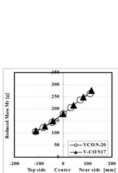
Fig. 22 Reduced mass at hitting locations of freely suspended racket
