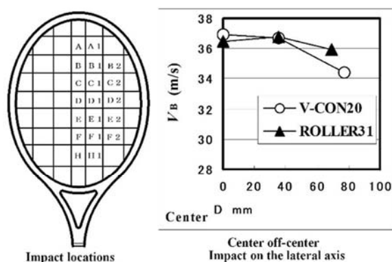
Fig. 18 Predicted post-impact ball velocity V_B ( N_s = 56.9 \text{ Nm} , V_{B0} = 10 \text{ m/s} )
