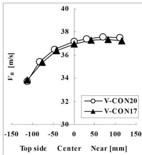
Fig. 26 Predicted post-impact ball velocity V_B ( N_s = 56.9 \text{ Nm} , V_{BO} = 10 \text{ m/s} , impact on the longitudinal axis).
