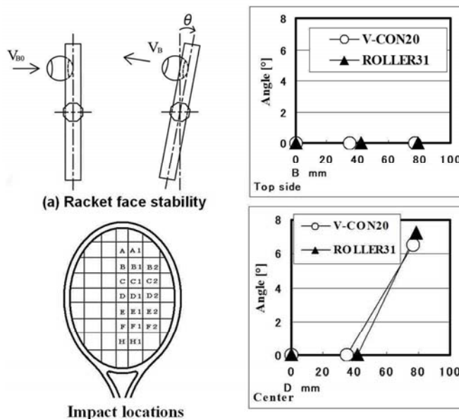
Fig. 19 Racket face rotation angle during ball contact (around the longitudinal axis)
