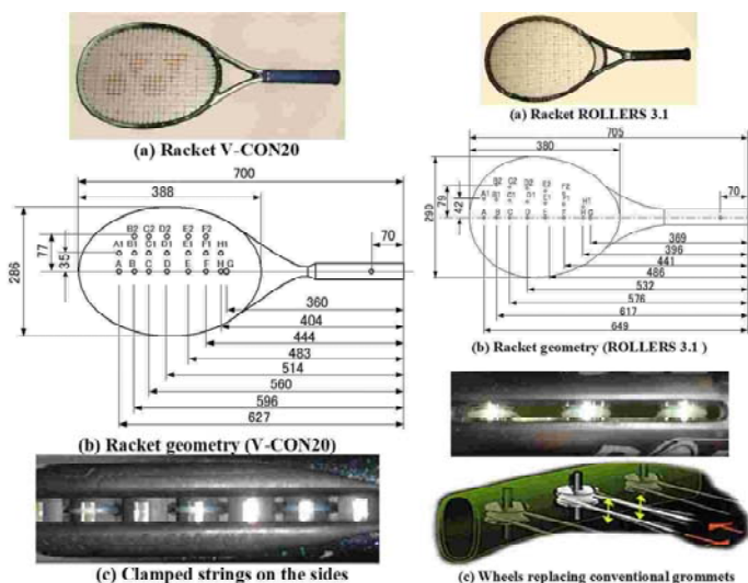
Fig. 13 Racket with clamped strings on the sides.
